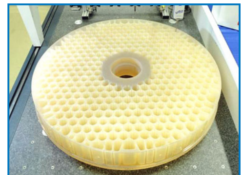
Backside of the 1.5 m diameter GREGOR Solar Telescope primary mirror
