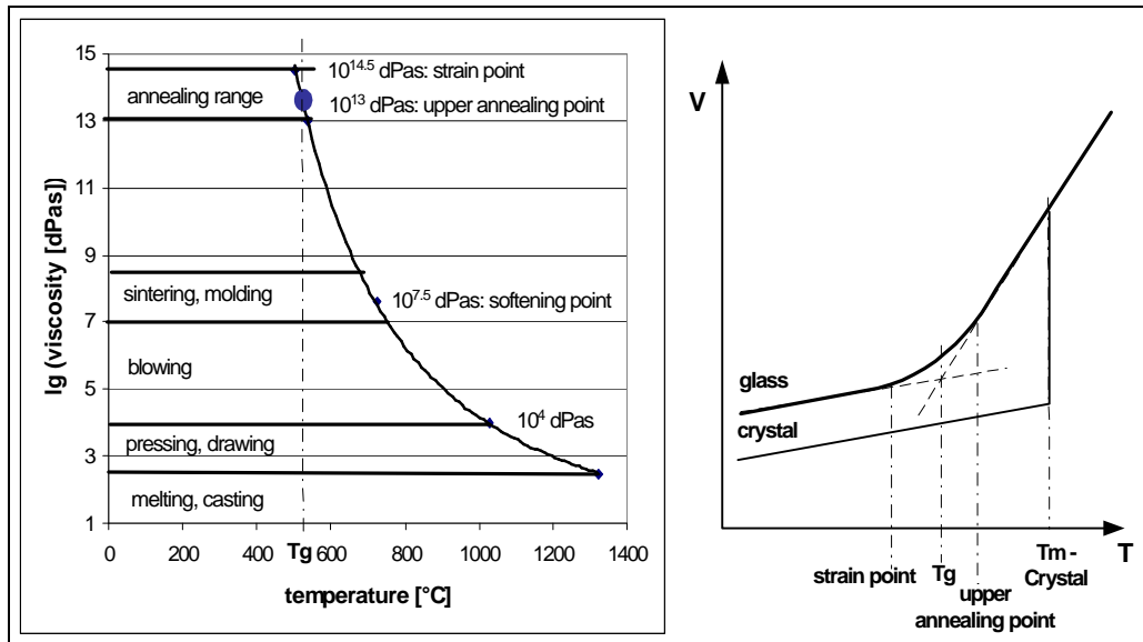
Figure 1: a) The viscosity of glass as a function of temperature. b) Tg definition in a Volume/Temperature diagram
