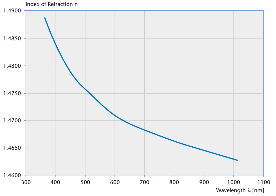
► Dispersion of BOROFLOAT® 33 – Index of Refraction n vs. Wavelength \lambda
