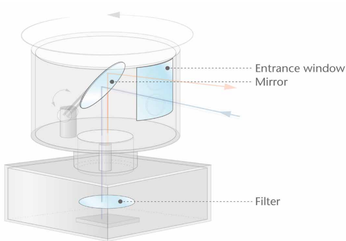
3 components of a traditional LiDAR unit could be made of BOROFLOAT® 33 borosilicate glass.
