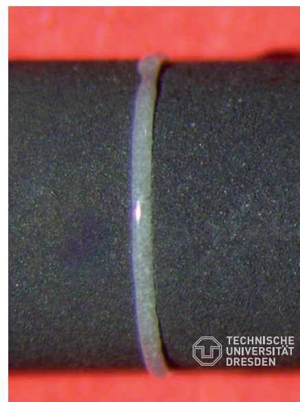
Joining of SiC ceramic with SCHOTT sealing glass.
